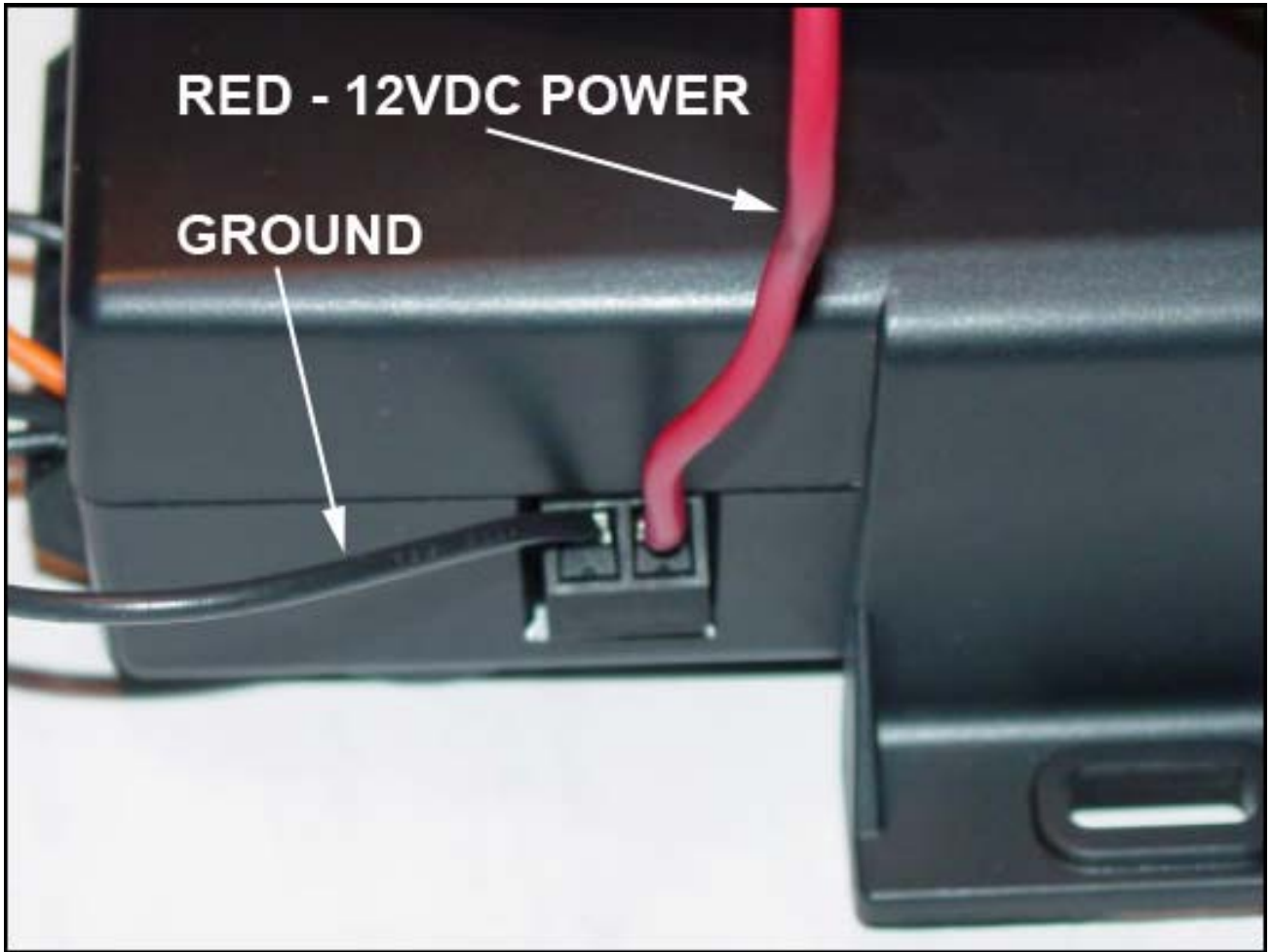
Figure 4. Power Connection to the LandAirSea 7100
