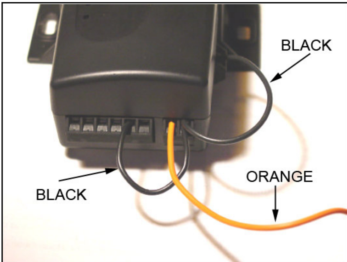
Figure 2. Control Wire Connection to LandAirSea 7100
