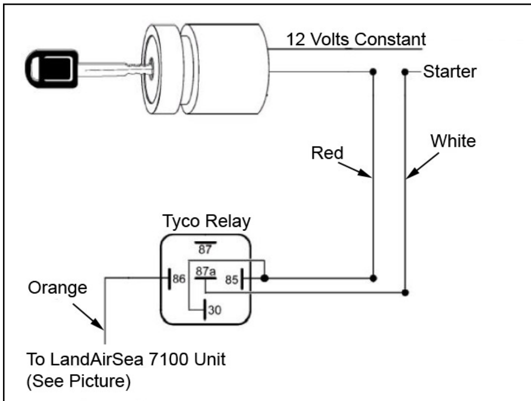
Figure 1. Wiring Diagram for the Starter Interrupt Relay
